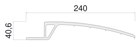
H35 running surface
